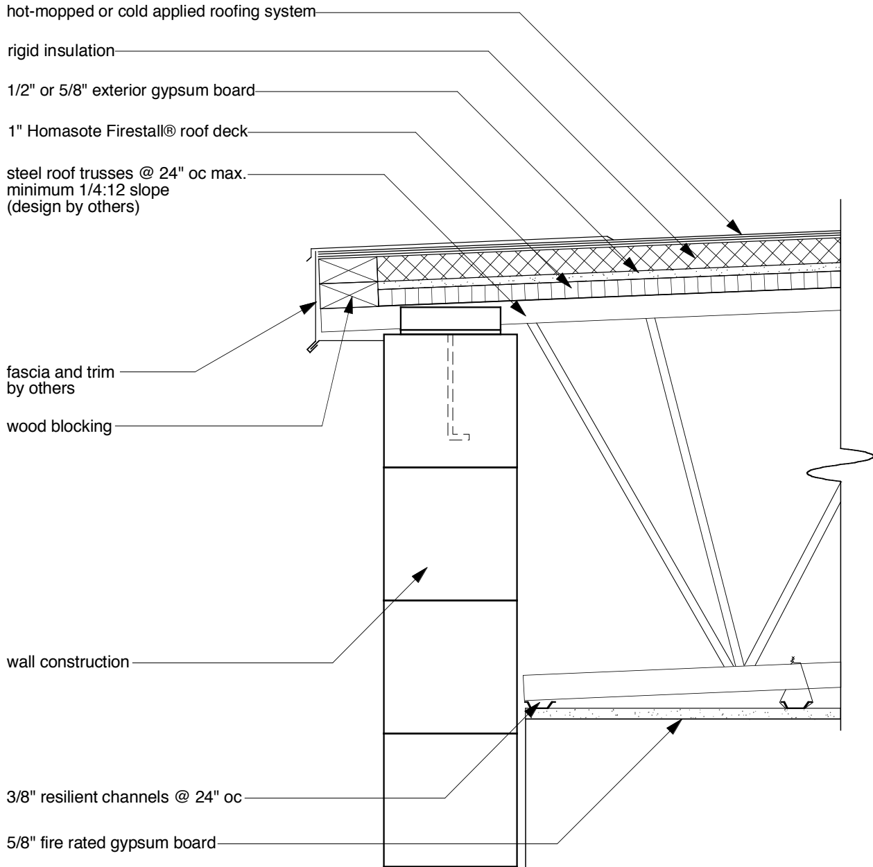
Firestall® Roof Deck Detail FS-HMCA-ID-1-24-5 UL Design No. P535
