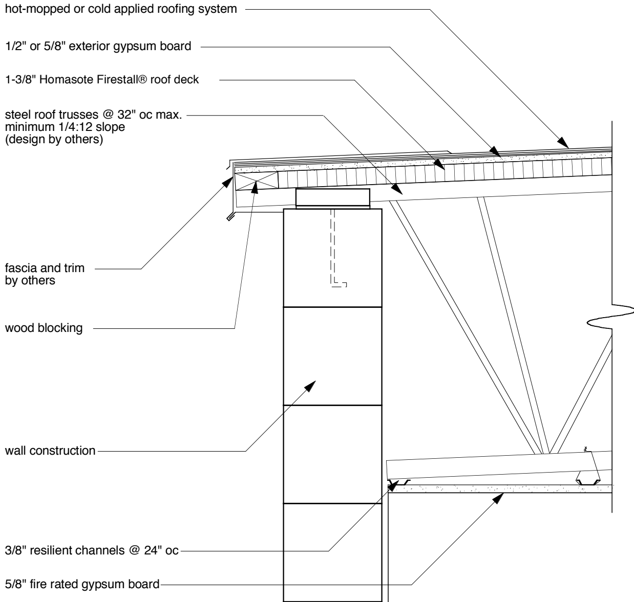
Firestall® Roof Deck Detail FS-HMCA-138-32-9 UL Design No. P535
