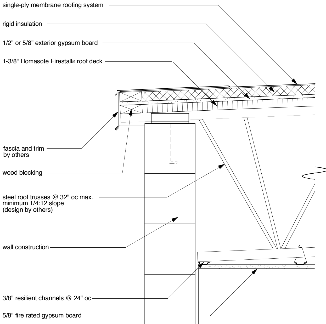
Firestall® Roof Deck Detail FS-SP-ID-138-32-14 UL Design No. P535
