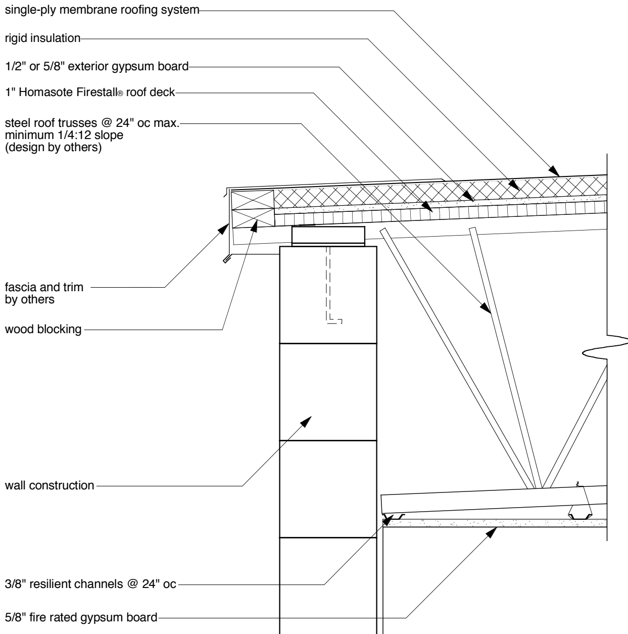
Firestall® Roof Deck Detail FS-SP-ID-1-24-6 UL Design No. P535
