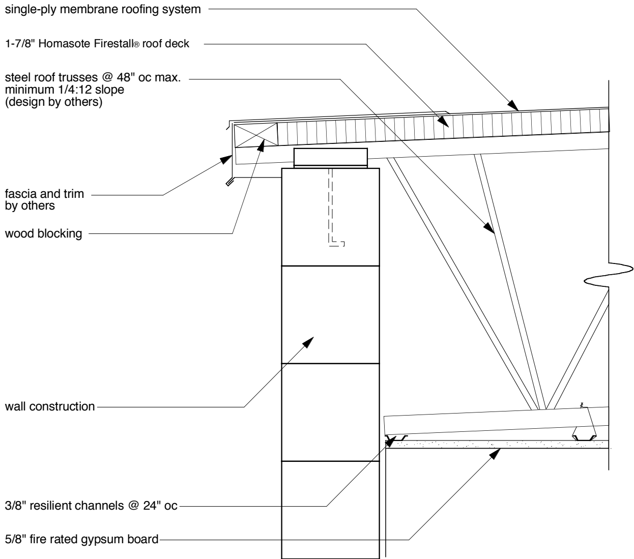
Firestall® Roof Deck Detail FS-SP-178-48-18 UL Design No. P535
