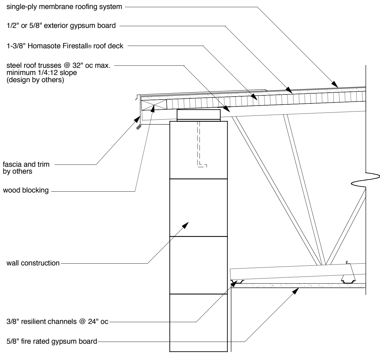
Firestall® Roof Deck Detail FS-SP-138-32-10 UL Design No. P535
