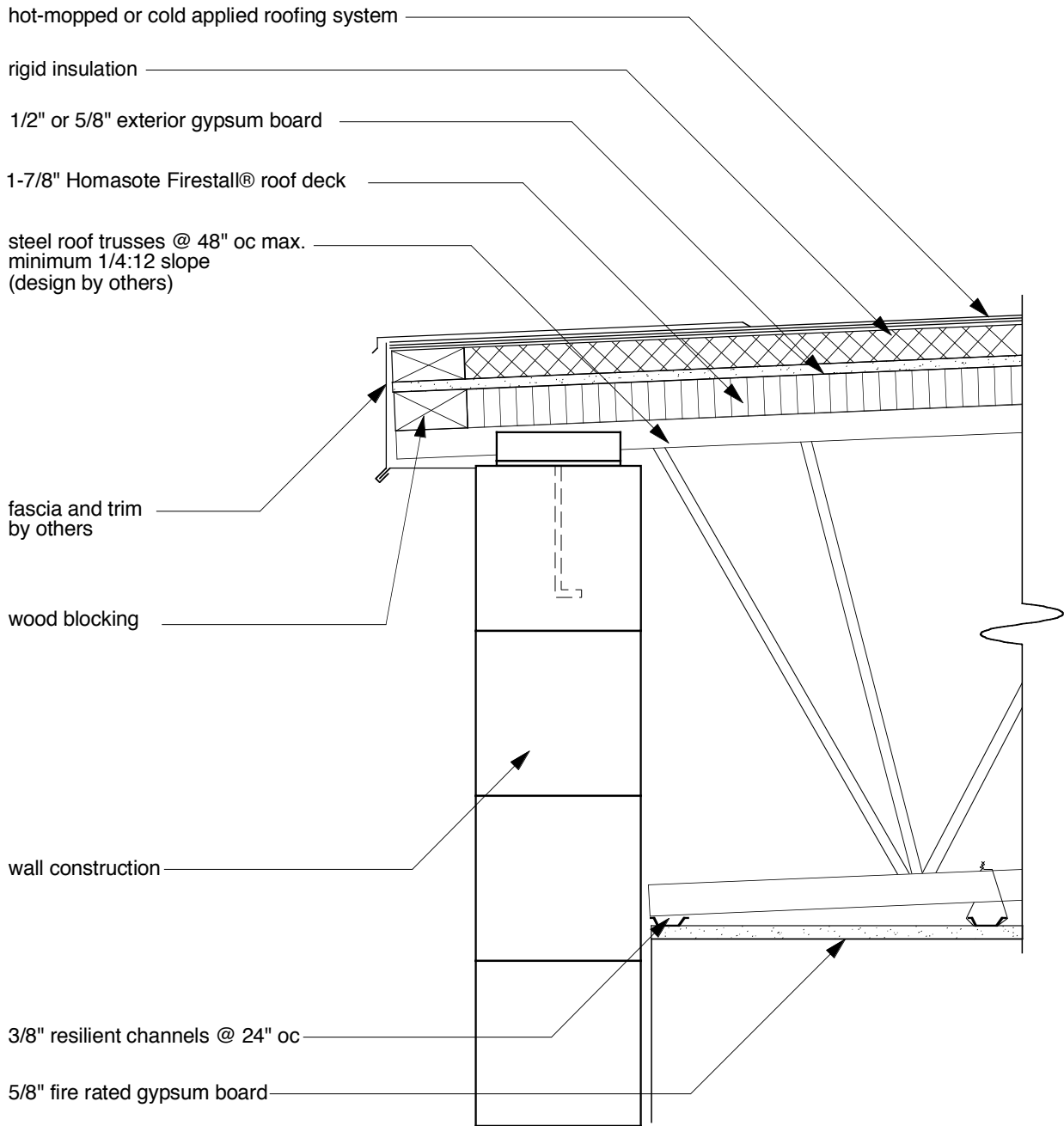
Firestall® Roof Deck Detail FS-HMCA-ID-178-48-25 UL Design No. P535
