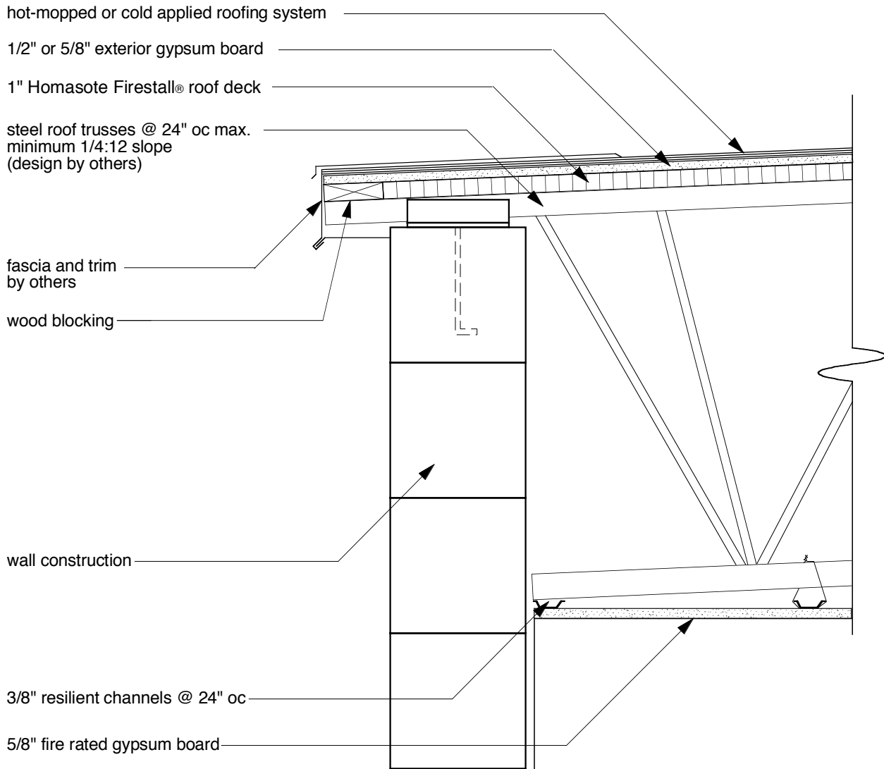
Firestall® Roof Deck Detail FS-HMCA-1-24-1 UL Design No. P535
